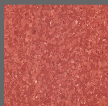
011 - Sunblaze - LRV-14
