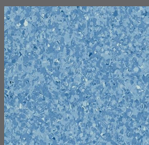
008 - Cloudburst - LRV-32
